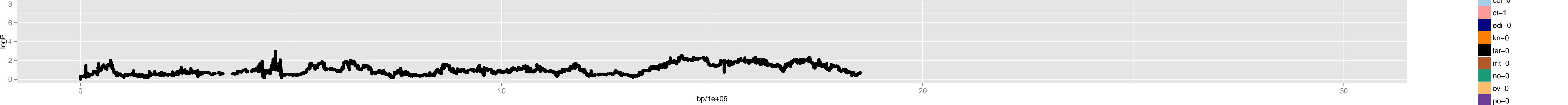
Chromosome 4 – Chr5_9600000
