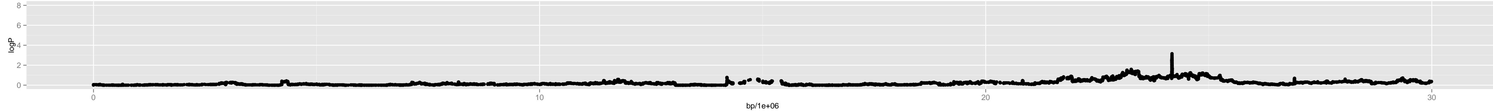
Chromosome 1 – Chr5_960000
