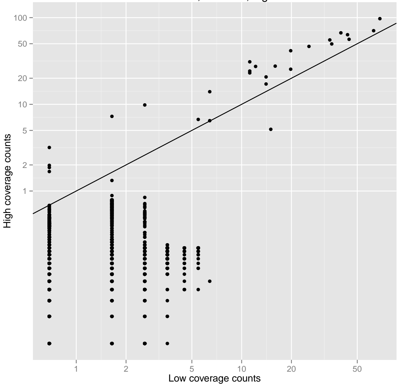
MAGIC.175 , r = 0.71 , logscale
