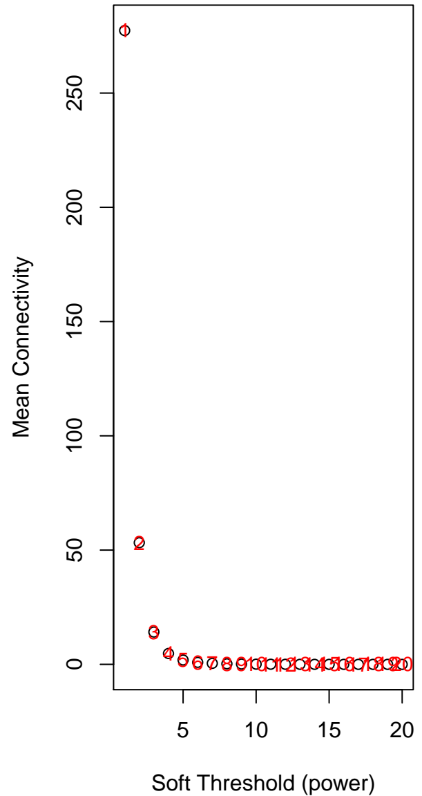
Mean connectivity
