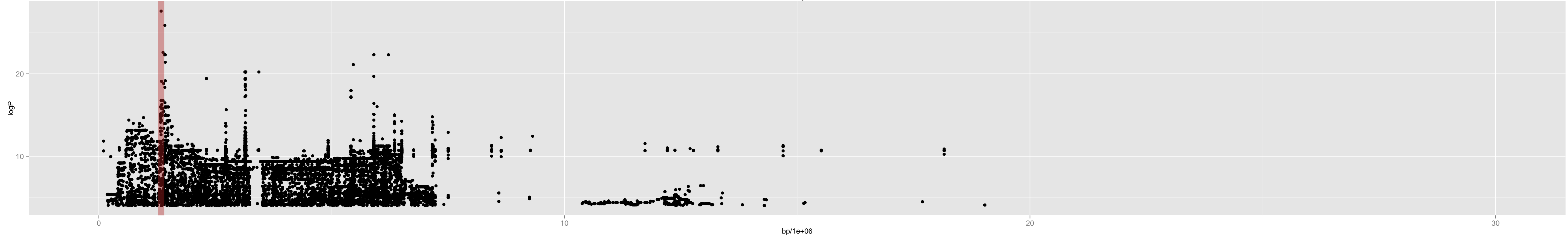
Chromosome 2 – 2_oy.0_1337447_10_1
