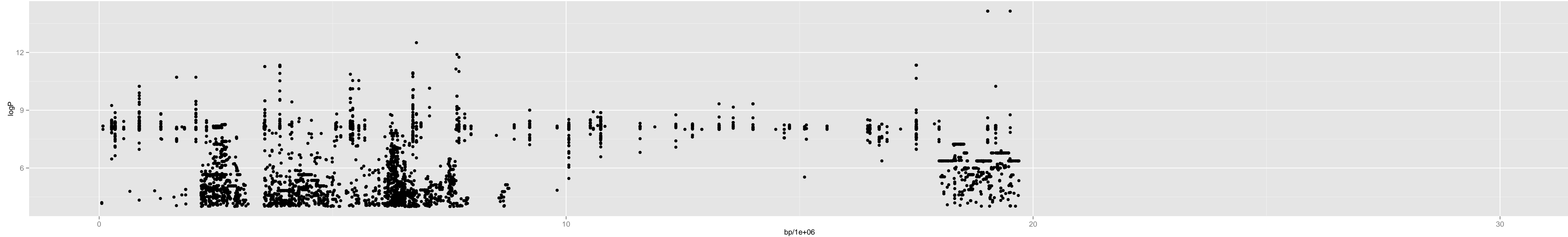
Chromosome 2 – 3_ws.0_12941409_13_10
