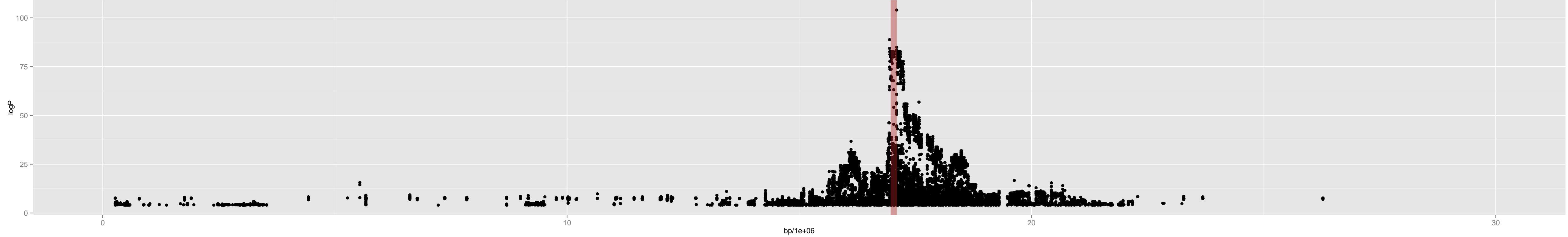
Chromosome 5 – 5_mt.0_17035475_14_5
