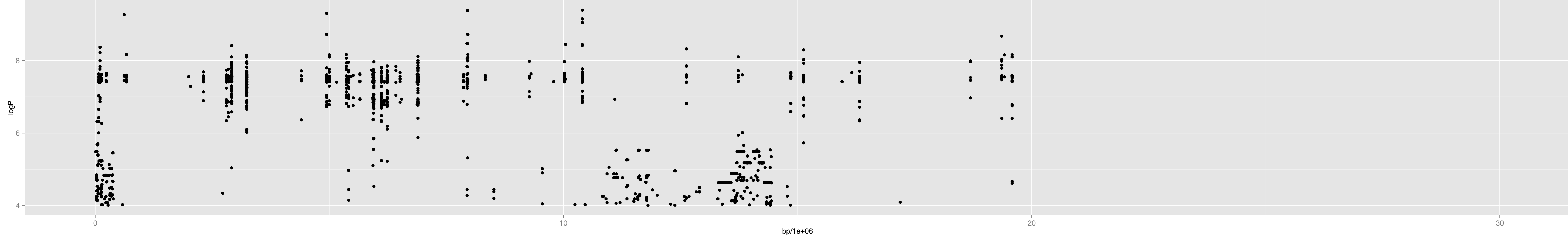
Chromosome 2 – 5_mt.0_17035475_14_5
