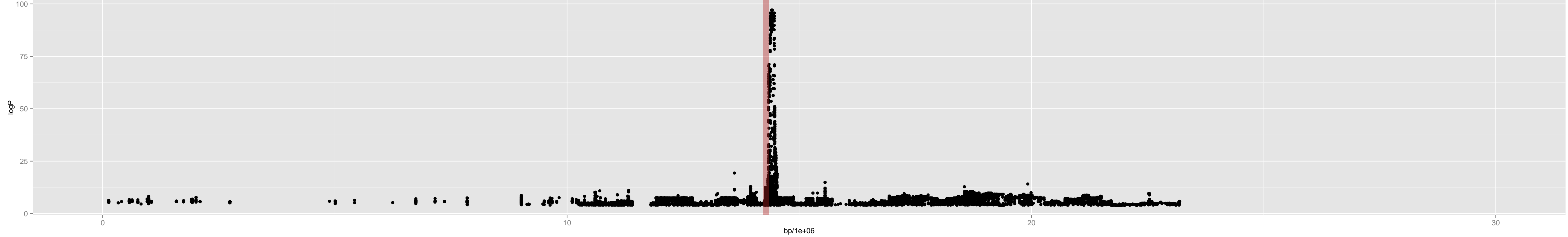
Chromosome 3 – 3_can.0_14285354_18_16
