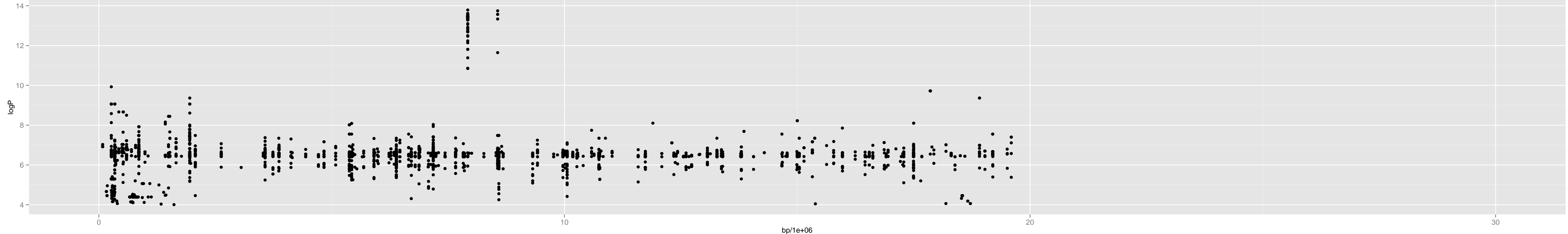
Chromosome 2 – 4_ler.0_4696358_16_6
