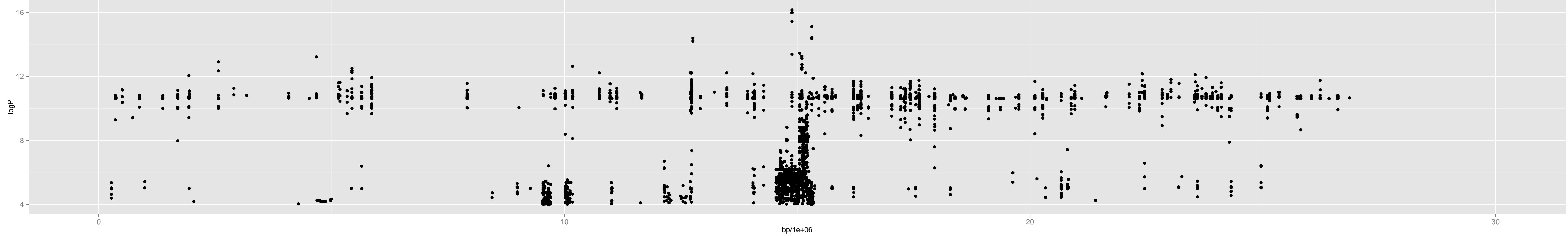
Chromosome 5 – 3_ler.0_14486922_10_5
