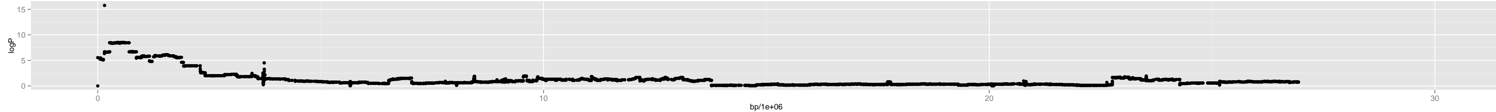
Chromosome 5 – 1_kn.0_9400943_5_2
