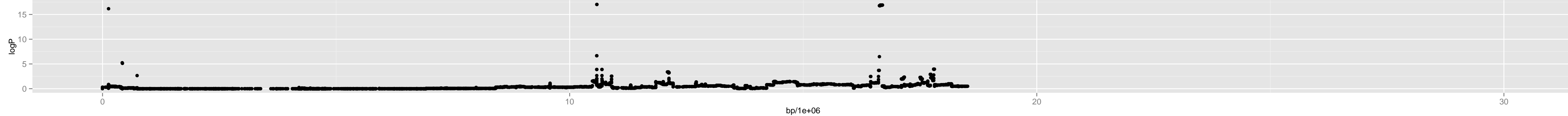
Chromosome 4 – 1_sf.2_6190763_5_5
