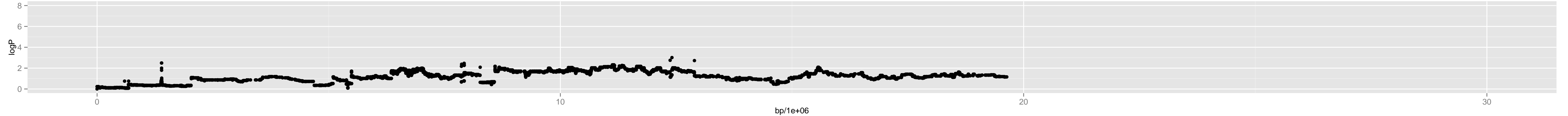
Chromosome 2 – 1_sf.2_6190763_5_5
