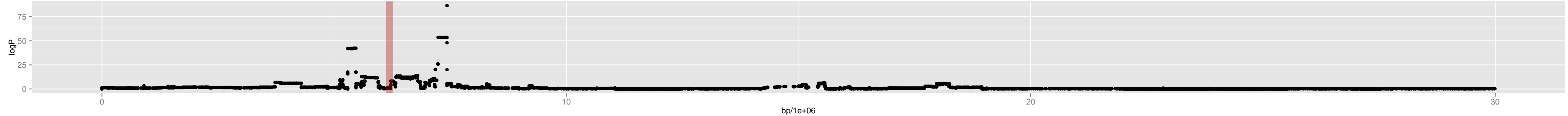
Chromosome 1 – 1_sf.2_6190763_5_5
