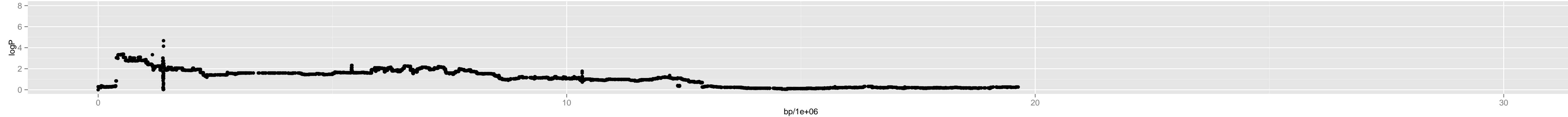
Chromosome 2 – 1_tsu.0_10246808_6_3
