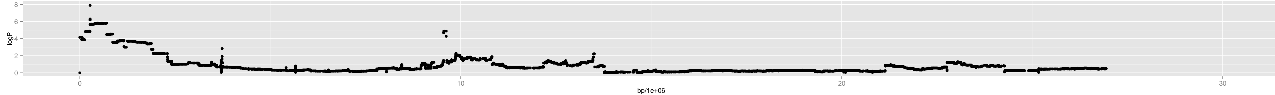
Chromosome 5 – 1_tsu.0_10246808_6_3
