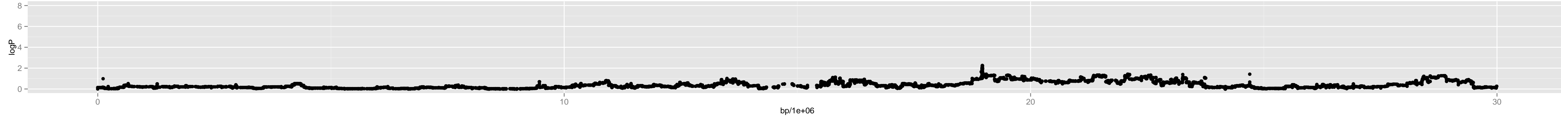
Chromosome 1 – 3_bur.0_14454399_36_12
