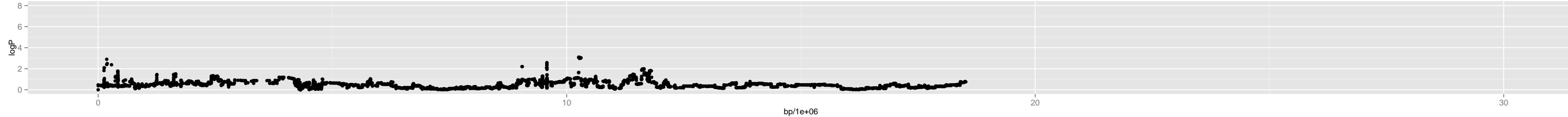
Chromosome 4 – 3_tsu.0_14303544_24_15
