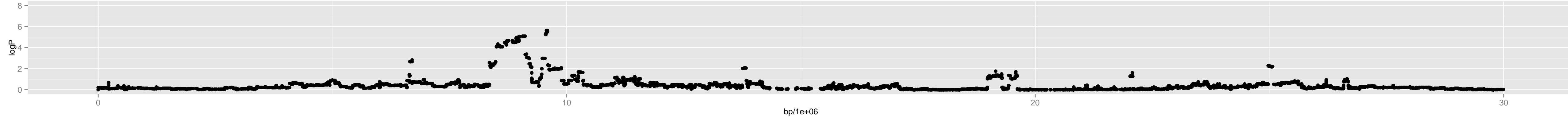
Chromosome 1 – 3_tsu.0_14303544_24_15
