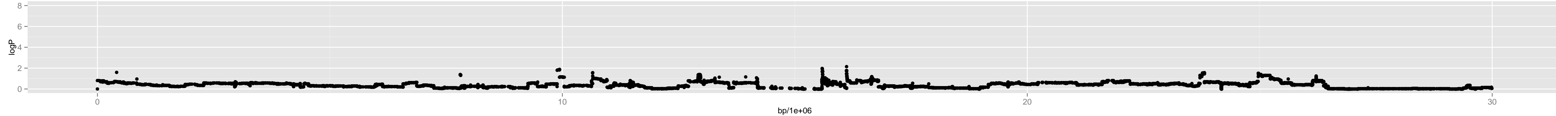
Chromosome 1 – 4_ct.1_4591718_13_7
