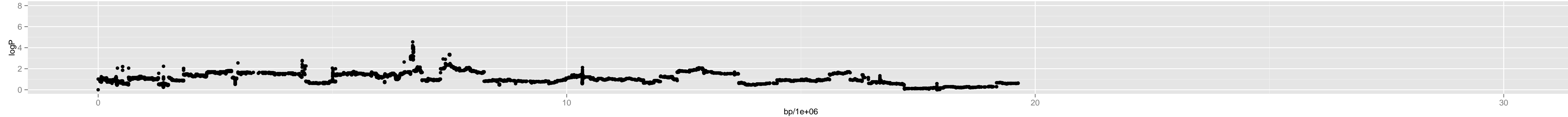
Chromosome 2 – 4_ct.1_4591718_13_7
