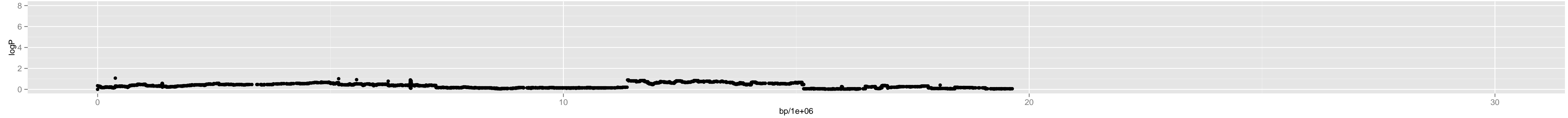
Chromosome 2 – 4_edi.0_4528569_6_6
