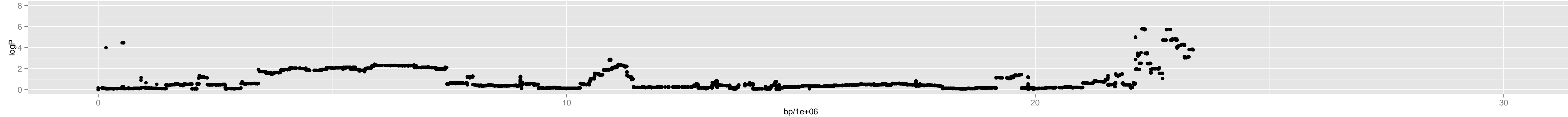
Chromosome 3 – 4_ler.0_13866739_6_4
