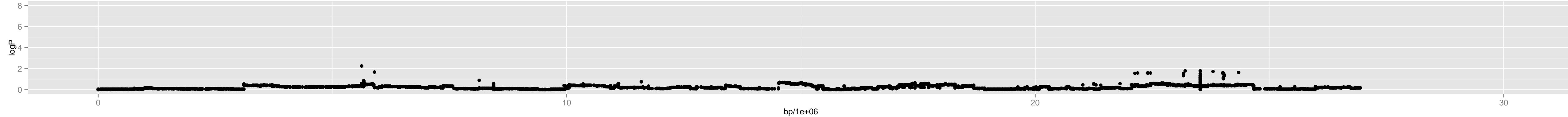
Chromosome 5 – 4_wil.2_1025_6_1
