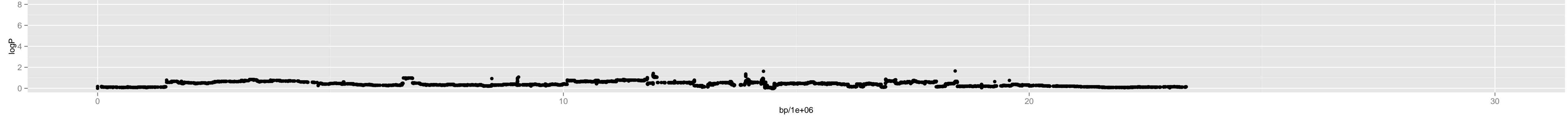
Chromosome 3 – 4_ws.0_4207737_5_5
