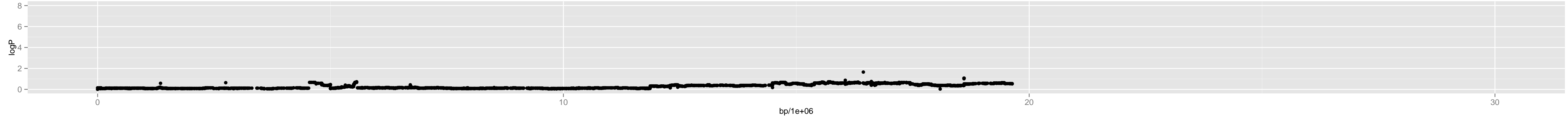
Chromosome 2 – 4_ws.0_4207737_5_5
