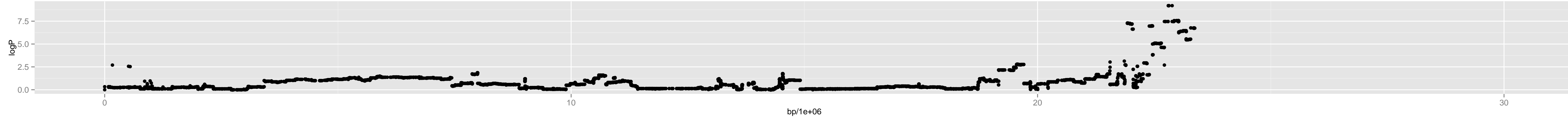
Chromosome 3 – 4_wu.0_13757353_9_3
