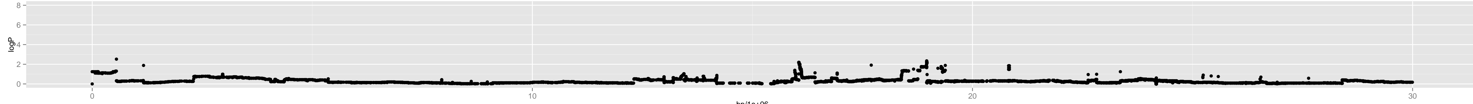
Chromosome 1 - 5_bur.0_12622819_5_5
