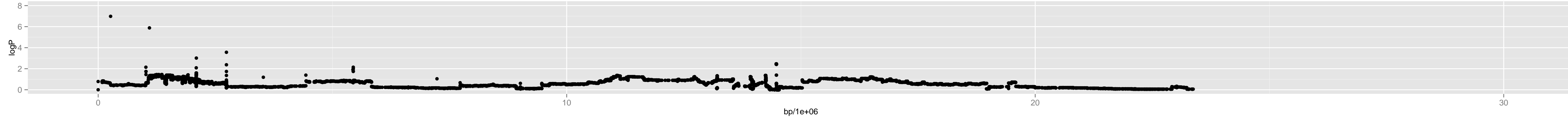
Chromosome 3 – 5_bur.0_12622819_5_5
