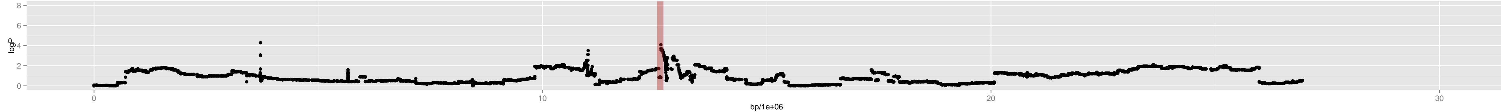
Chromosome 5 – 5_bur.0_12622819_5_5
