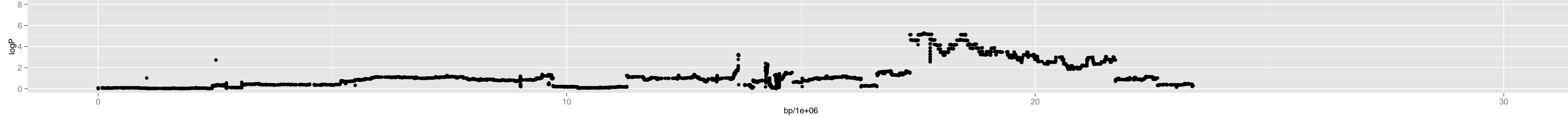
Chromosome 3 – 5_mt.0_58_5_1
