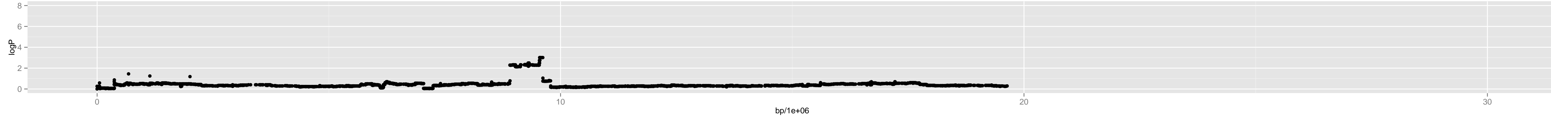
Chromosome 2 – 5_mt.0_58_5_1
