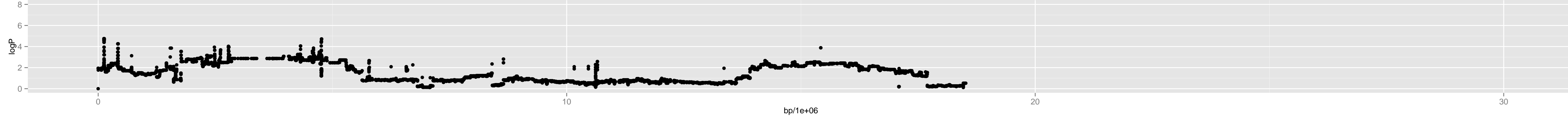
Chromosome 4 – 5_mt.0_58_5_1
