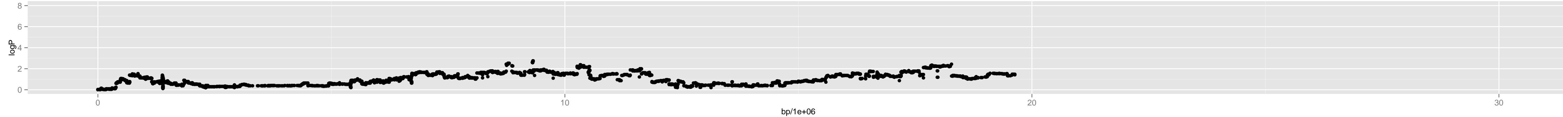
Chromosome 2 – 1_zu.0_11433867_23_3
