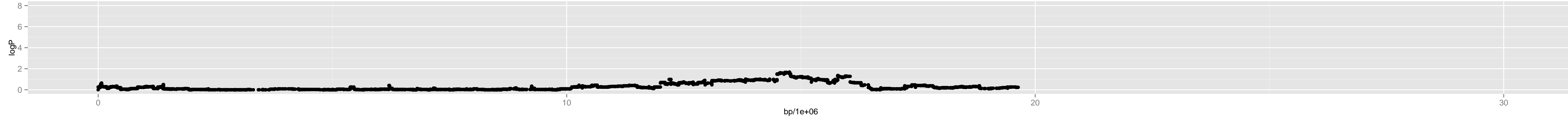
Chromosome 2 – 3_sf.2_14328742_27_25
