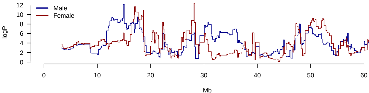
Imm.PctCD8inCD3 Chromosome 19
