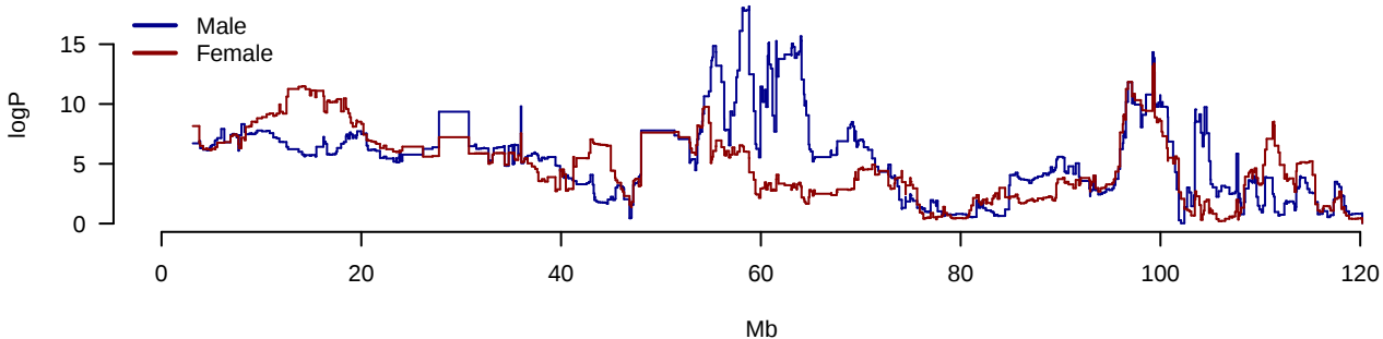
Imm.PctCD8inCD3 Chromosome 14
