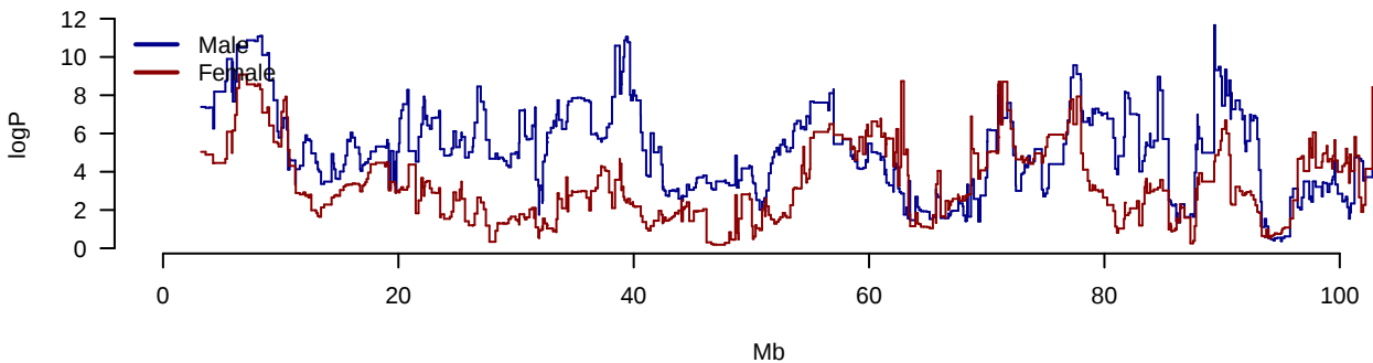
Imm.PctCD8inCD3 Chromosome 15
