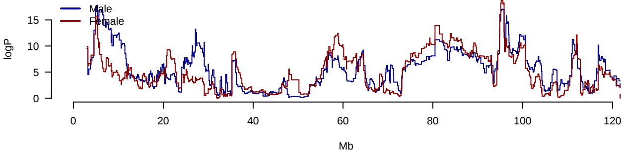
Imm.PctCD8inCD3 Chromosome 12
