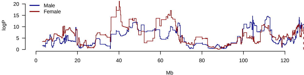
Imm.PctCD8inCD3 Chromosome 11
