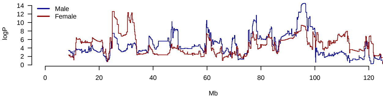
Imm.PctCD8inCD3 Chromosome 14
