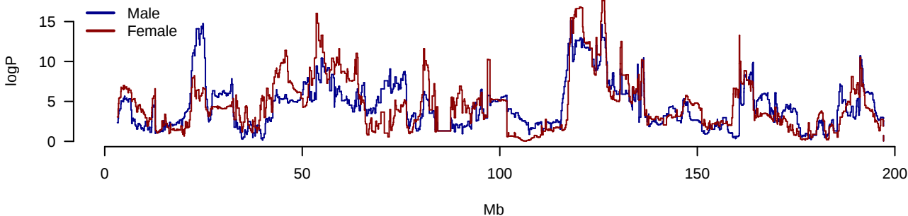
Imm.PctCD8inCD3 Chromosome 2
