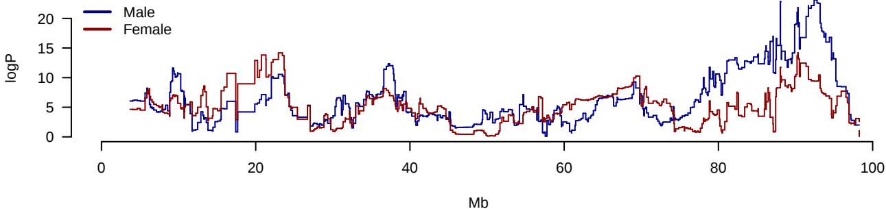
Imm.PctCD8inCD3 Chromosome 17
