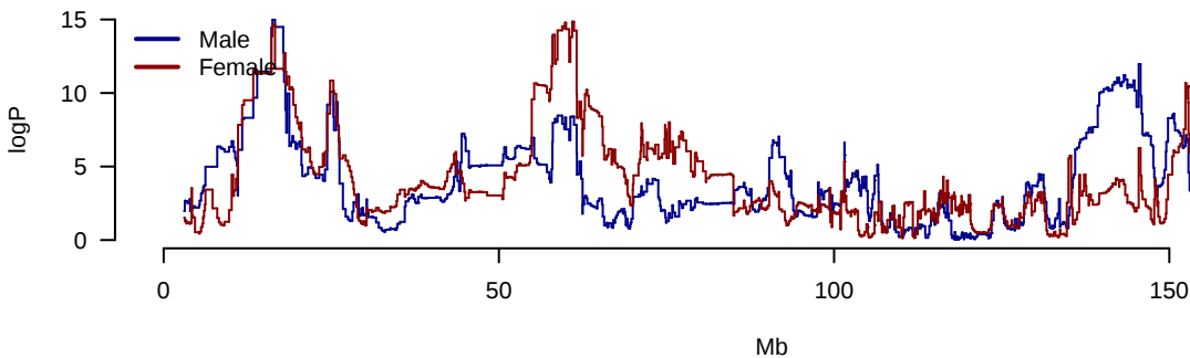
Imm.PctCD8inCD3 Chromosome 2
