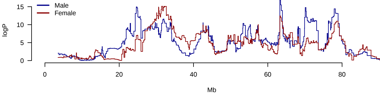
Imm.PctCD8inCD3 Chromosome 18
