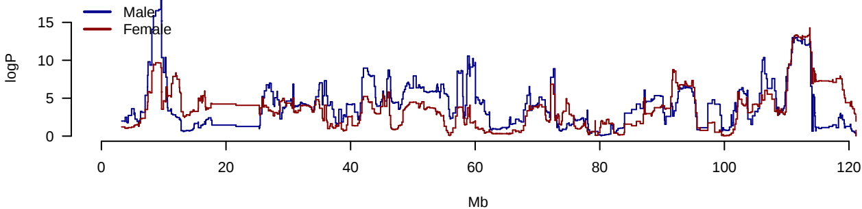
Imm.PctCD8inCD3 Chromosome 12
