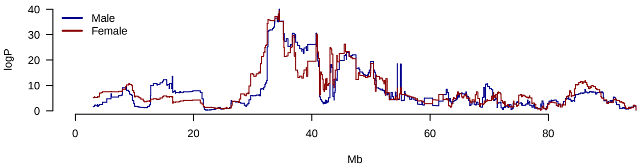
Imm.PctCD8inCD3 Chromosome 17
