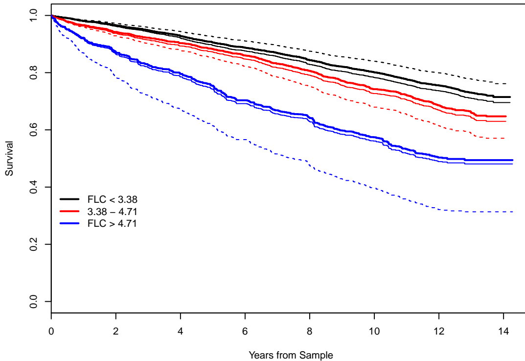
Figure 4: Survival curves for the three groups using reweighted data are shown with solid lines, the original unweighted analysis as dashed lines. The heavier solid line adjusts to the Olmsted population and the lighter one to the US population.
