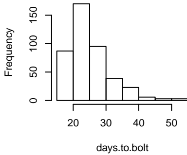
days.to.bolt
