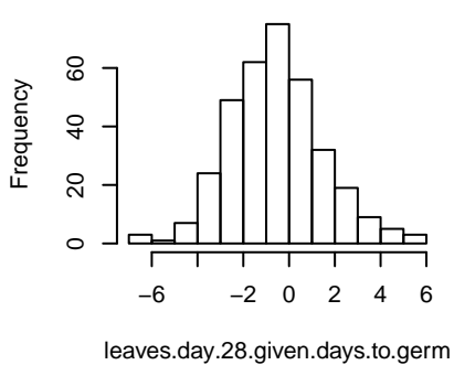
leaves.day.28.given.days.to.germ
