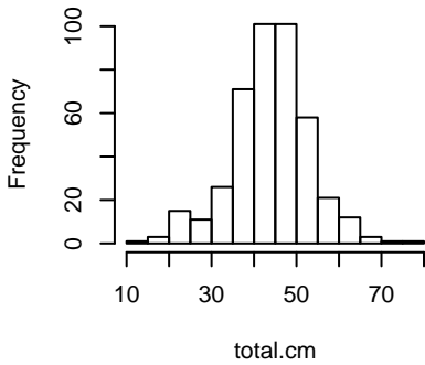
total.cm
