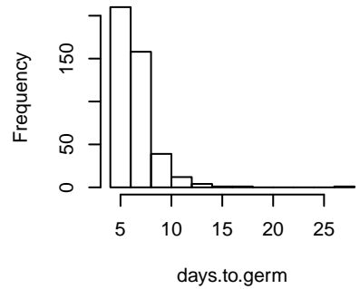
days.to.germ
