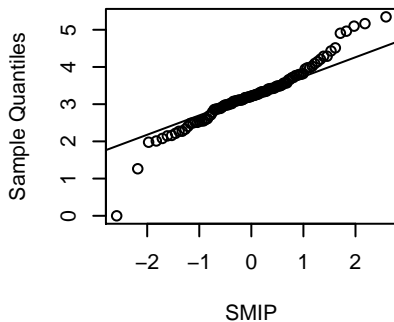
SMIP
