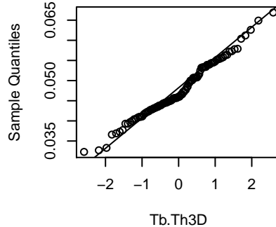
Tb.Th3D
