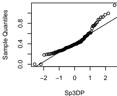
Sp3DP
