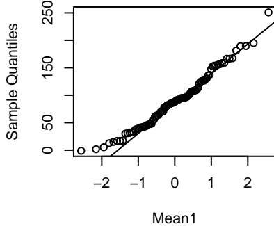
Mean1
