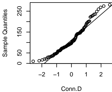
Conn.D
