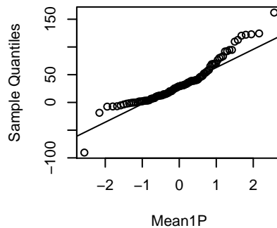
Mean1P
