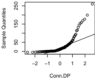
Conn.DP
