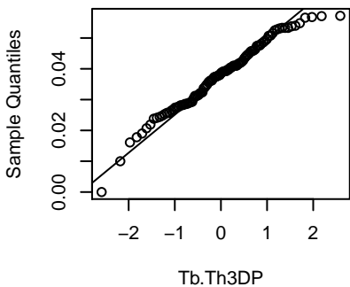
Tb.Th3DP
