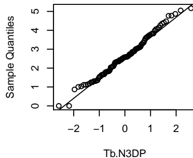
Tb.N3DP
