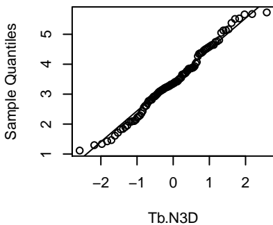
Tb.N3D
