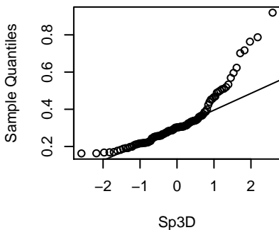
Sp3D
