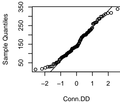
Conn.DD
