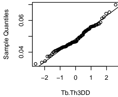
Tb.Th3DD
