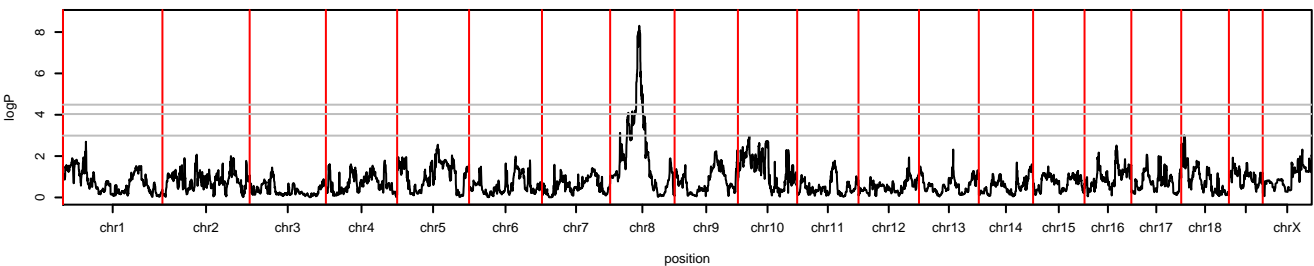
Tb.N.met
