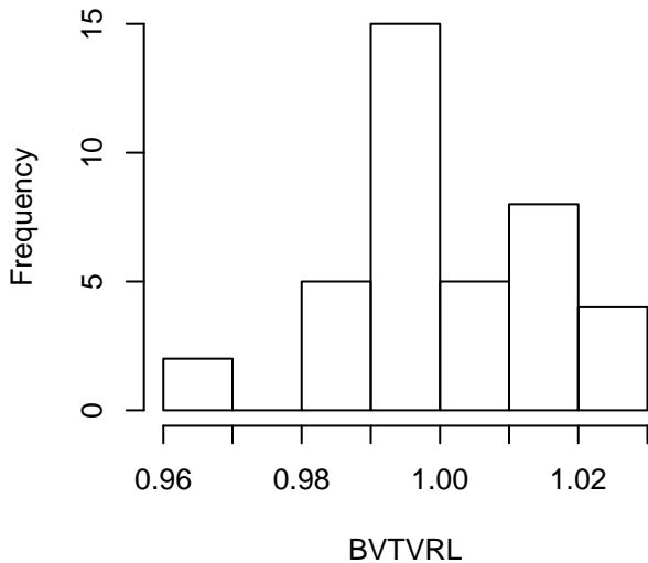
Histogram of df1[[i]]
