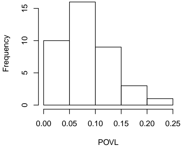
Histogram of df1[[i]]
