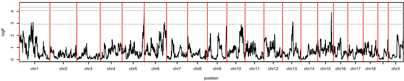
TbND
