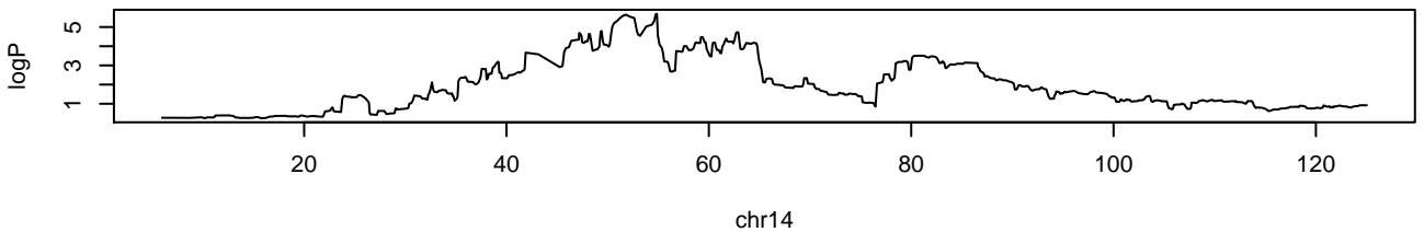
raw-16-4-2014_JOINT.weighted.RData chr14 54772473 5.68 0.002
