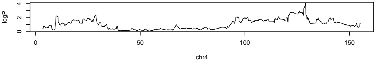
raw-16-4-2014_JOINT.weighted.RData chr4 128898346 4.04 0.094
