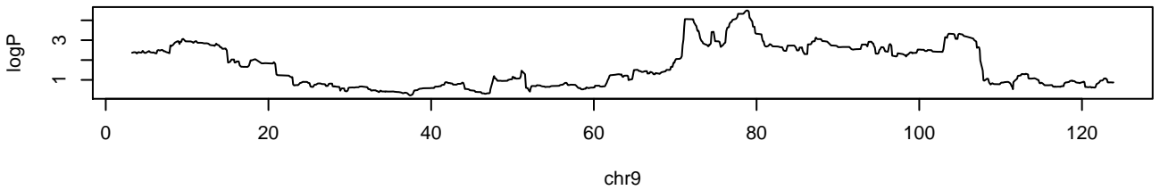
raw-16-4-2014_JOINT.weighted.RData chr9 78772467 4.5 0.042
