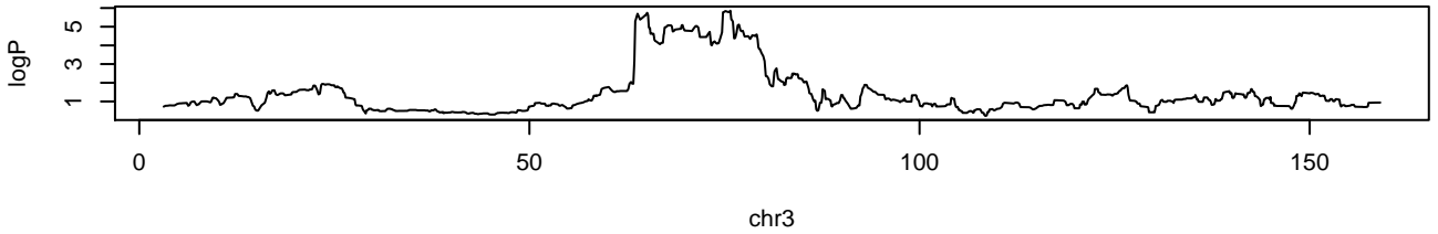
raw-16-4-2014_JOINT.weighted.RData chr3 75706779 5.86 0
