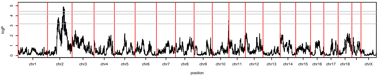
recomb.score
